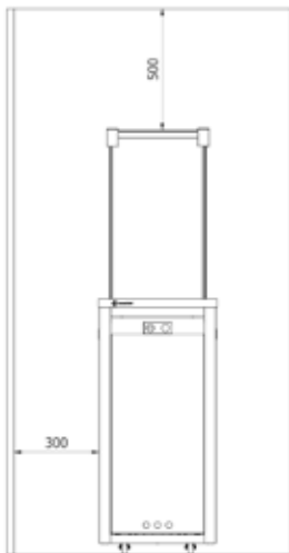
Fig. Minimum clearance from flammable materials/objects
